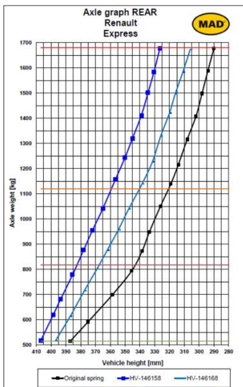
Coil suspension characteristic
