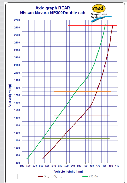
Power Spring Characteristic HV-314325
