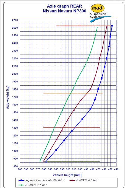
Air Suspension Characteristic
