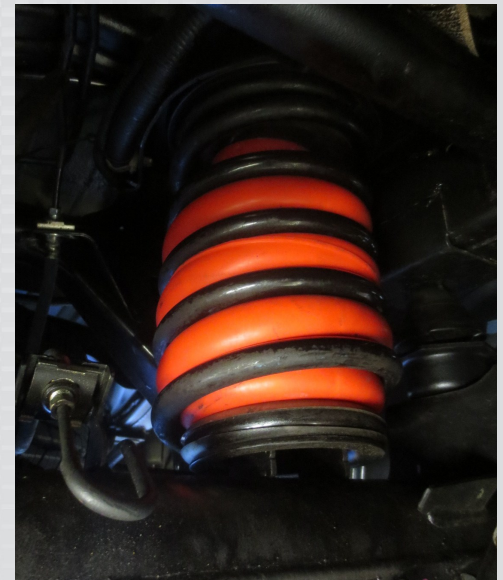
Airbellow in Original Rear Coil Spring
